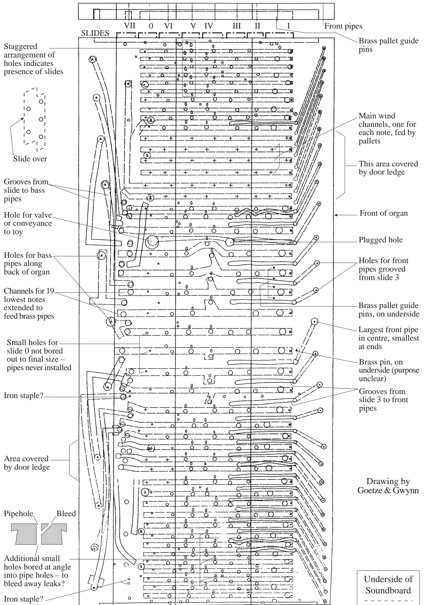
Measured drawing of the Wetheringsett soundboard, with principal features annotated
